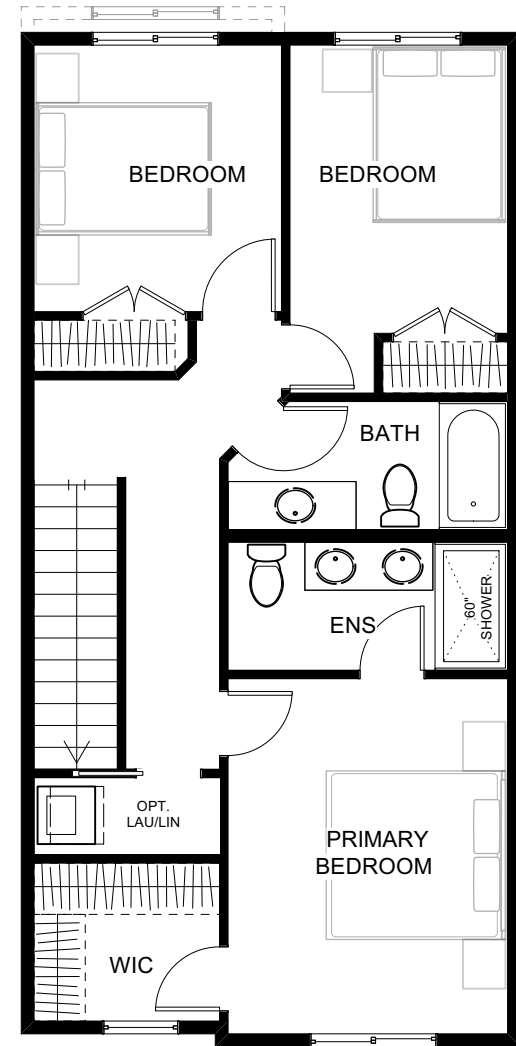
UPPER FLOOR
